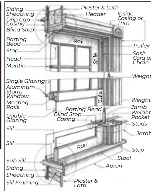
Anatomy of a Double-Hung Window, adapted from Jonathan Poore
